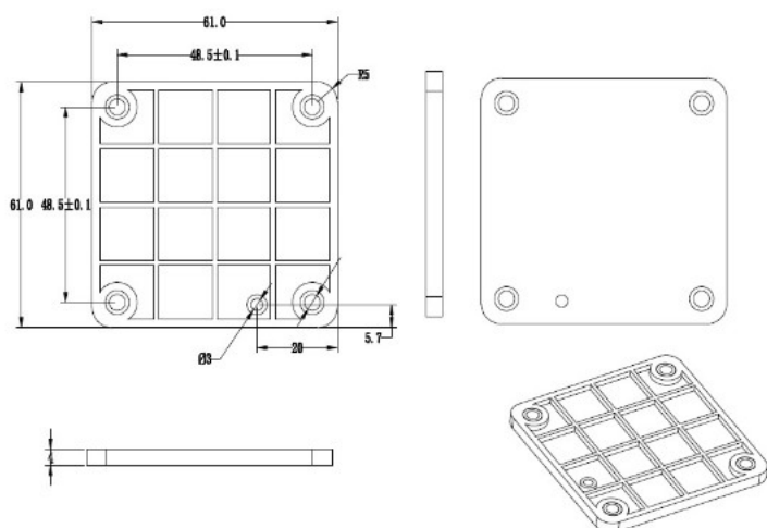
Back Plate F/Lock
